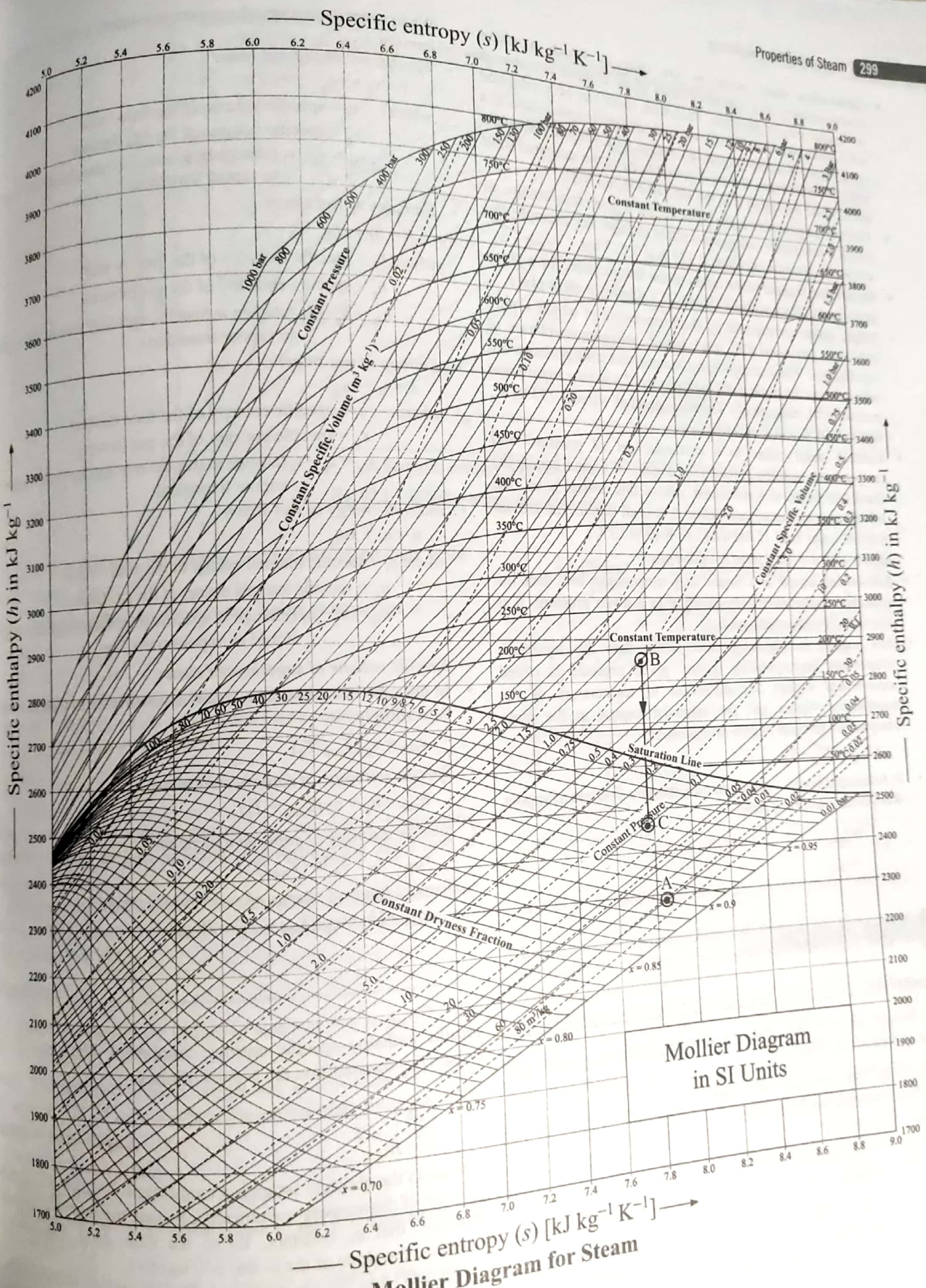
Fig. 7.18 Mollier Diagram for Steam
